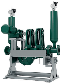
Sludge Pro® Double Disc Pump
